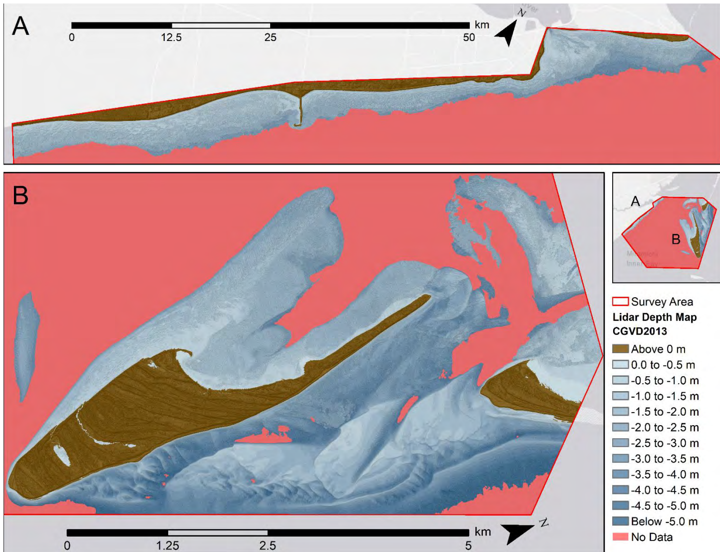
Figure 14. Depth contour map showing depth contours every 0.5 m to a depth of 5 m.
