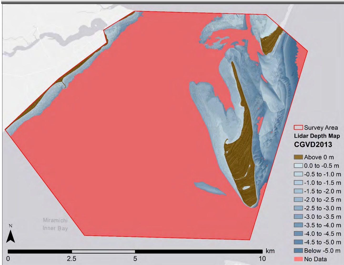
Figure 4. Lidar coverage map of the Miramichi Inner Bay area. Signal extinction occurred at 6.85 m depth which was shallower than the large central portion of the bay.
