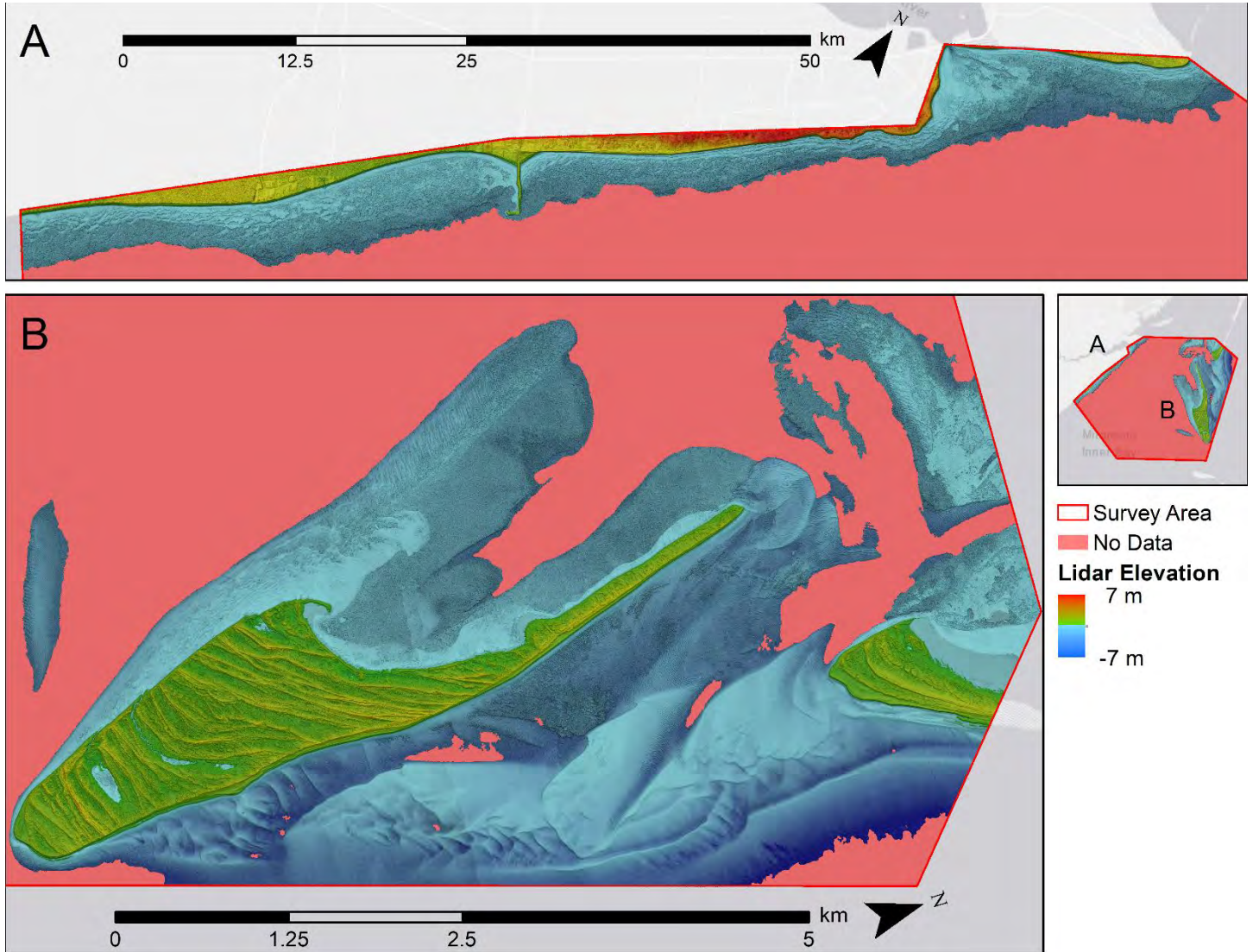
Figure 12. Colour shaded relief model of the study area. The DEM CSR shows the separation of land and water at 0 m CGVD2013 at the blue-green boundary.
