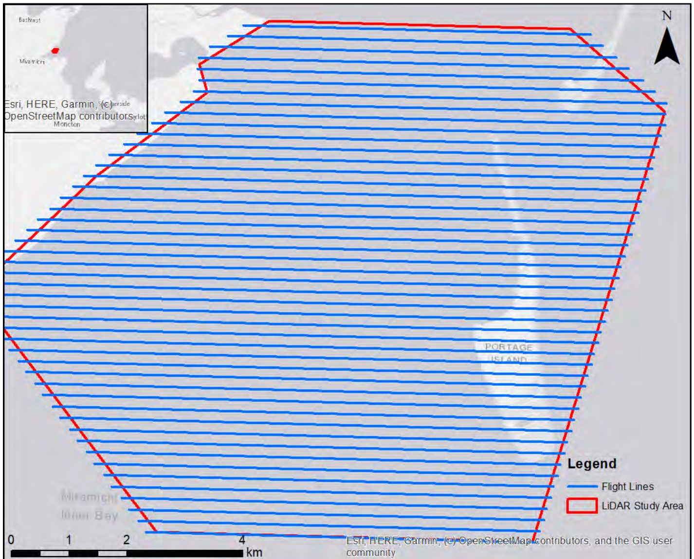
Figure 1. Globe study area and planned flight lines over Burnt Church, NB.
