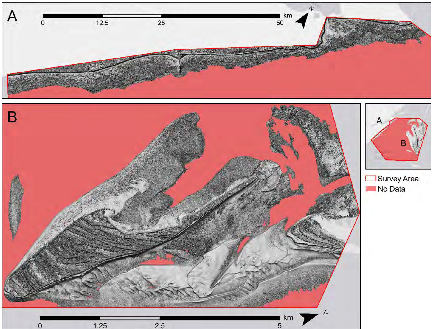
Figure 11. Seamless topo-bathy digital elevation model of Burnt Church, NB with 50 times vertical exaggeration.
