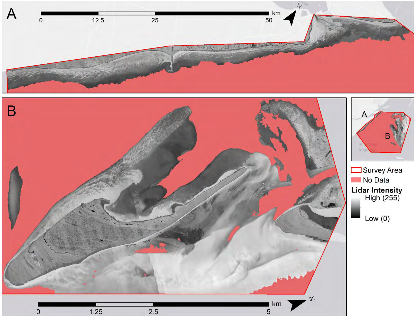
Figure 13. Depth normalized intensity map which separates highly absorbent materials, like eelgrass, from highly reflective materials, such as sand, regardless of depth.
